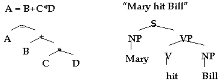
Figure 7. Analysis of a sentence
