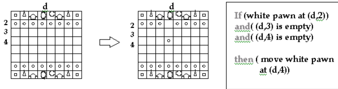
Figure 4. A chess move is being codified as a set of logical predictions.
